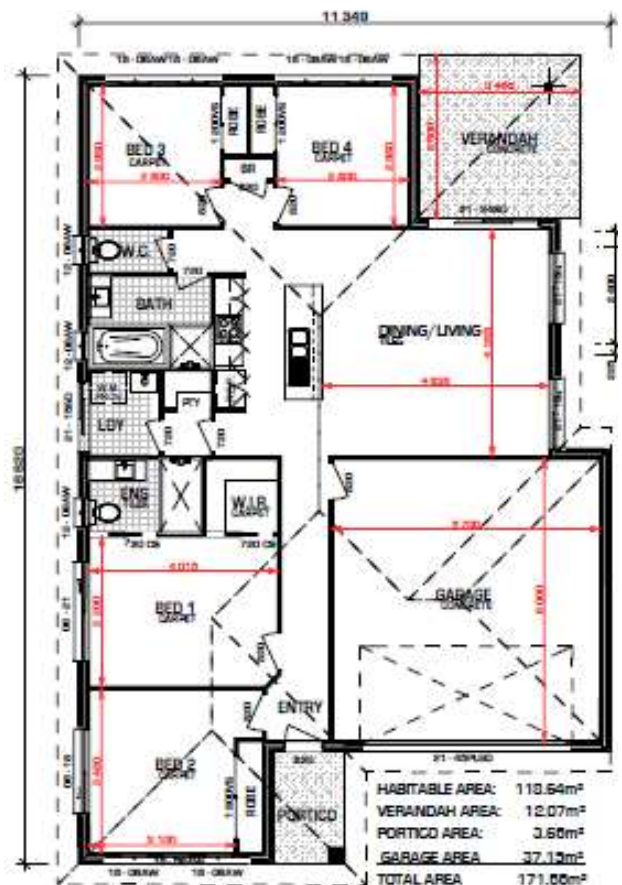
FLOOR PLAN 1:100
